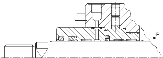
Standard bush
