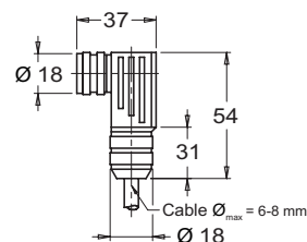
7 pins DIN metal connector with 90° square, adjustable direction female coupling
